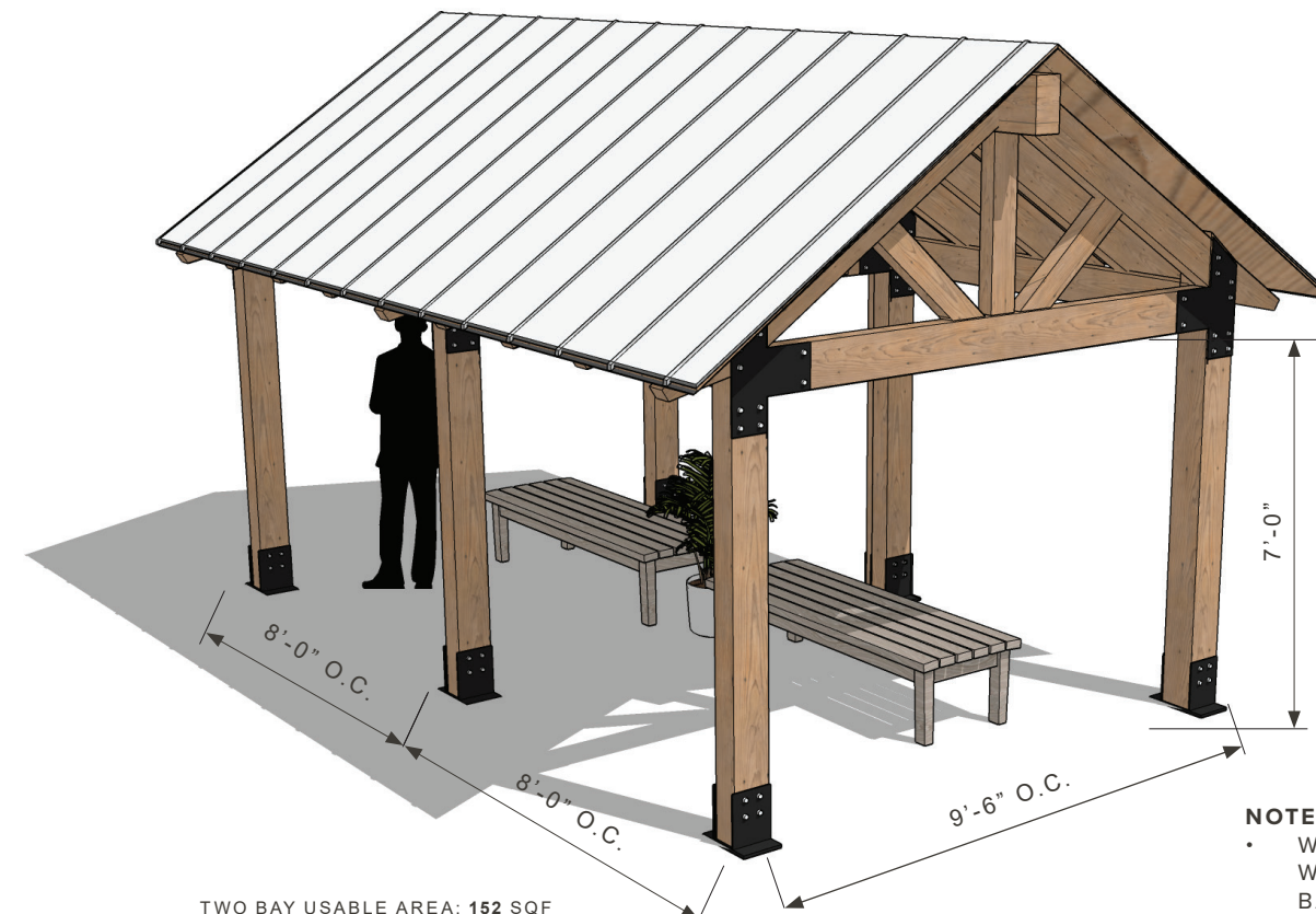
TWO BAY VERSION OF SHADE STRUCTURE (AXON)VIEW
