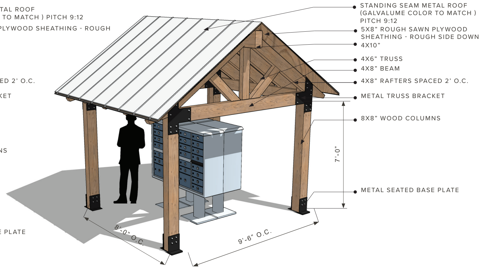
ONE BAY VERSION OF SHADE STRUCTURE (AXON)VIEW
